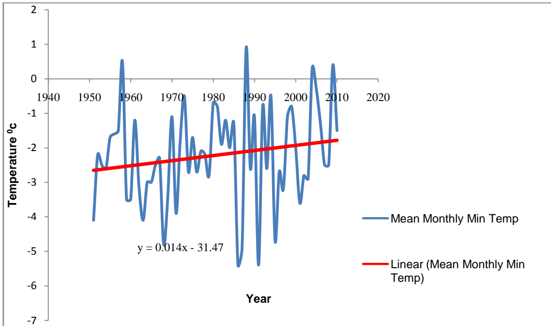
Figure 2: Core-Winter Mean Monthly Minimum Temperature of Srinagar from (1950 – 2010)
